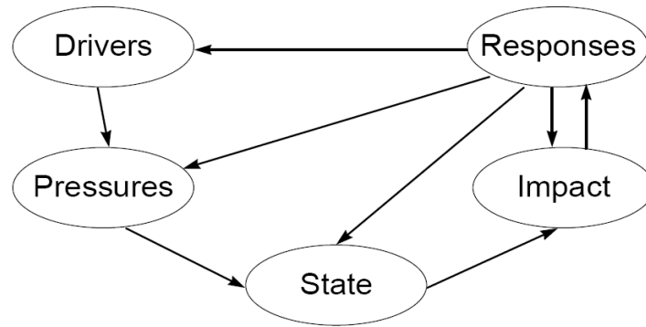
Fig. 1 The Driving forces, Pressures, State, Impacts, Responses framework.
