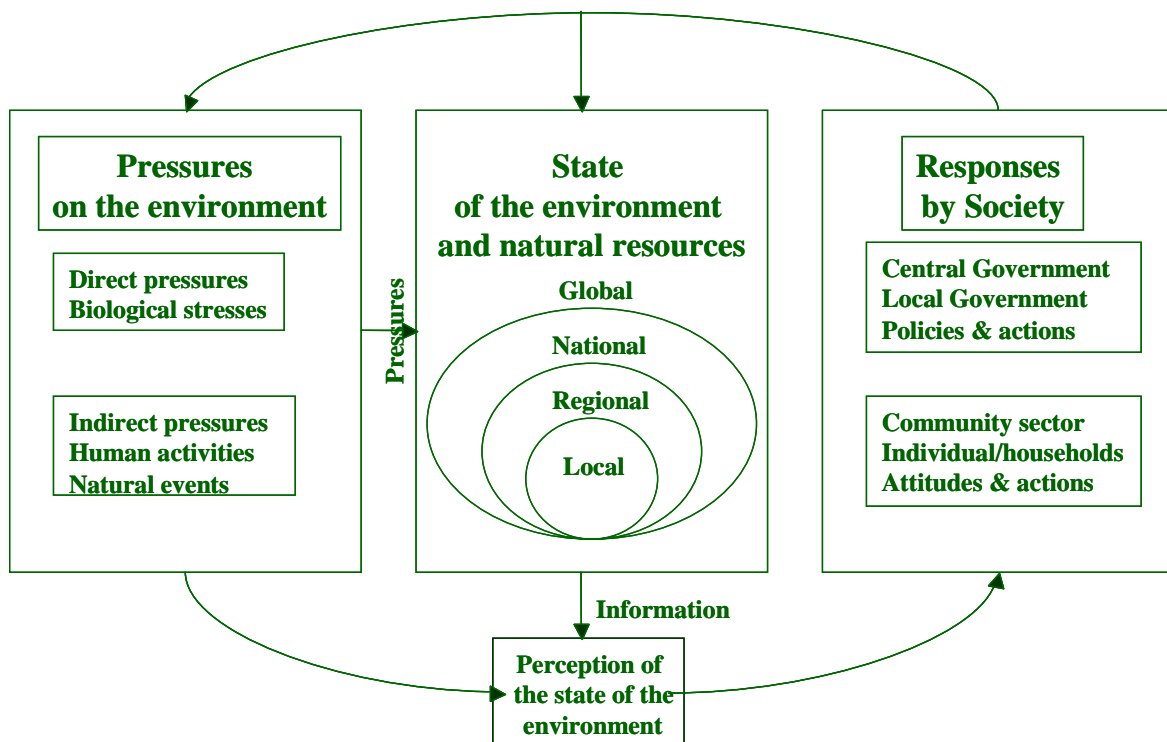
Fig. 2. Pressure-State-Response framework for environmental reporting
