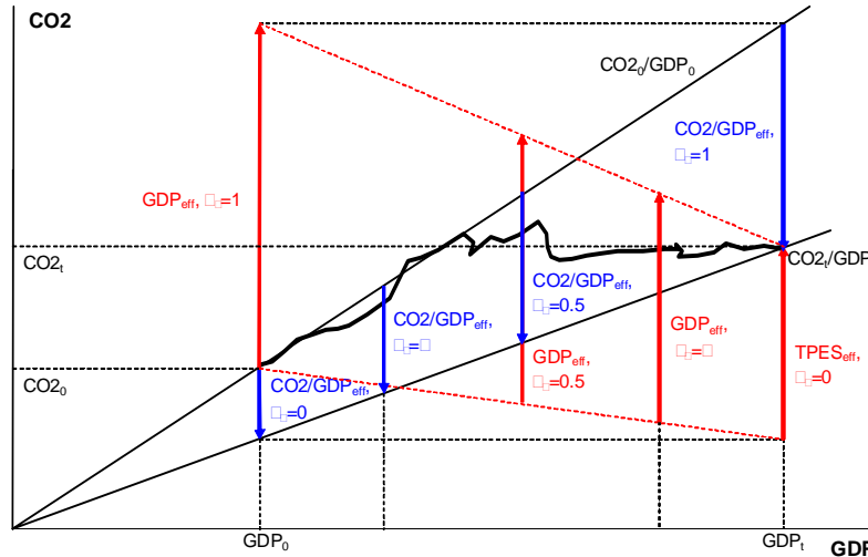
Fig. 3: Decomposition of CO2 change: the effects of CO2/GDP and GDP during a selected time period
