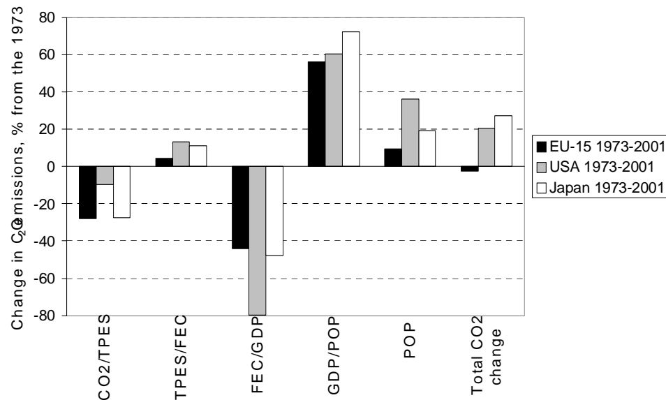
Fig. 4. ASA of the change in CO 2 emissions from fuel combustion in the EU-15, in the USA, and in Japan 1973–2001. Data source: International Energy Agency
